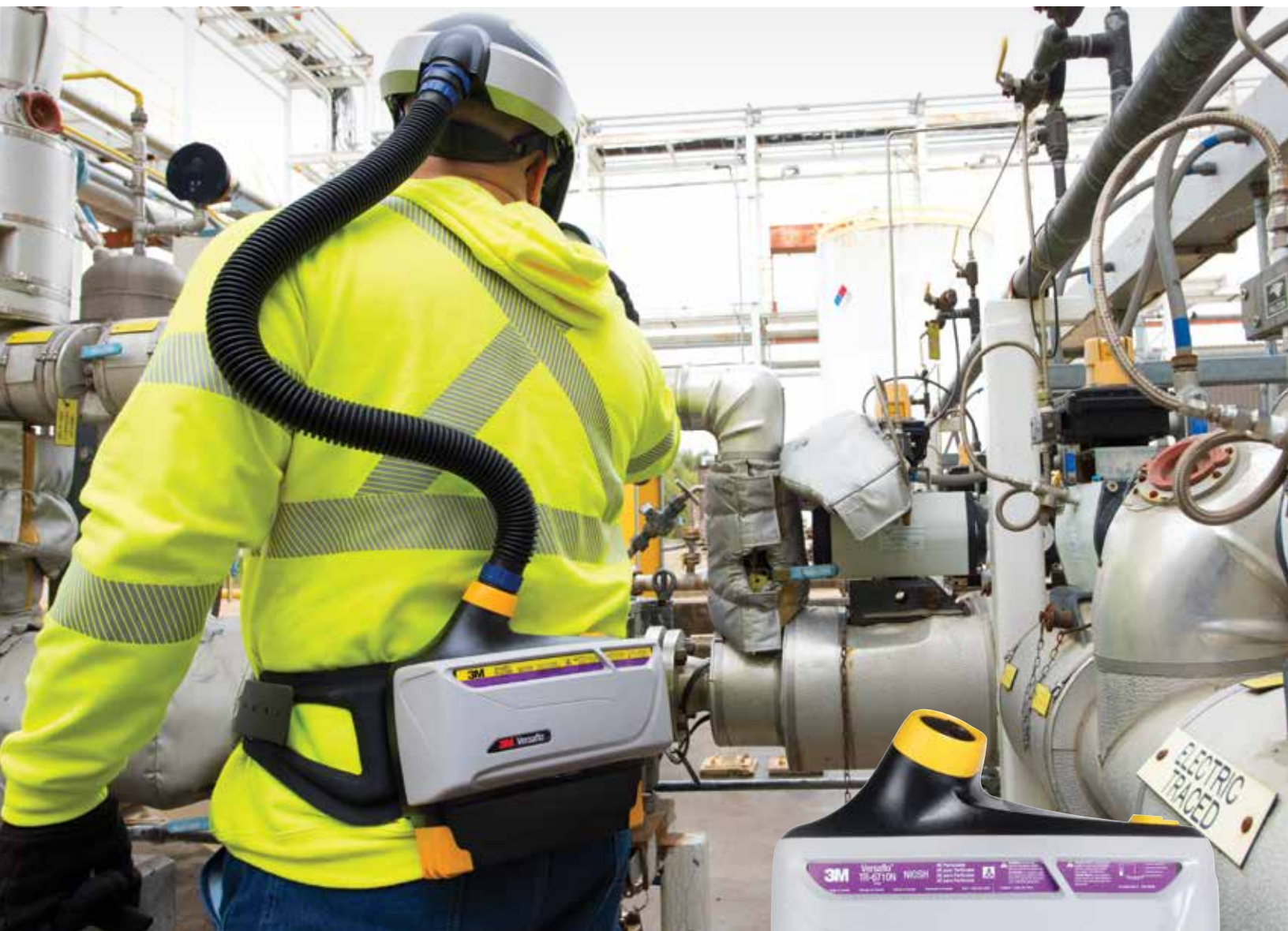
3M™ Versaflo™ TR-800 Intrinsically Safe Powered Air Purifying Respirator
